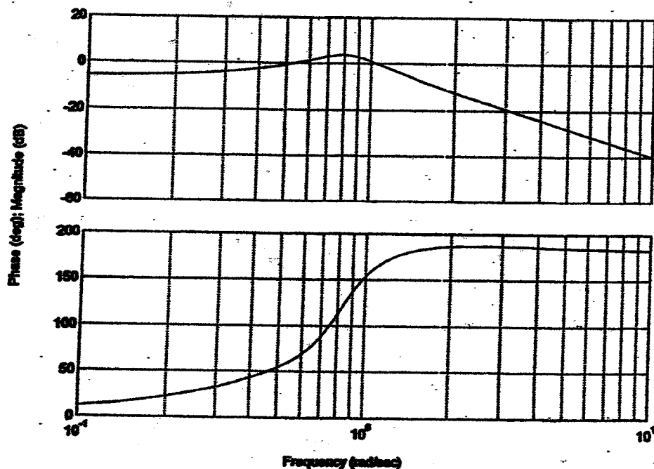
Bode Diagram of G(s) = (s+0.5)/(s^3+s^2+1)
