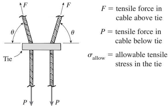
FREE-BODY DIAGRAM OF HALF THE TIE
