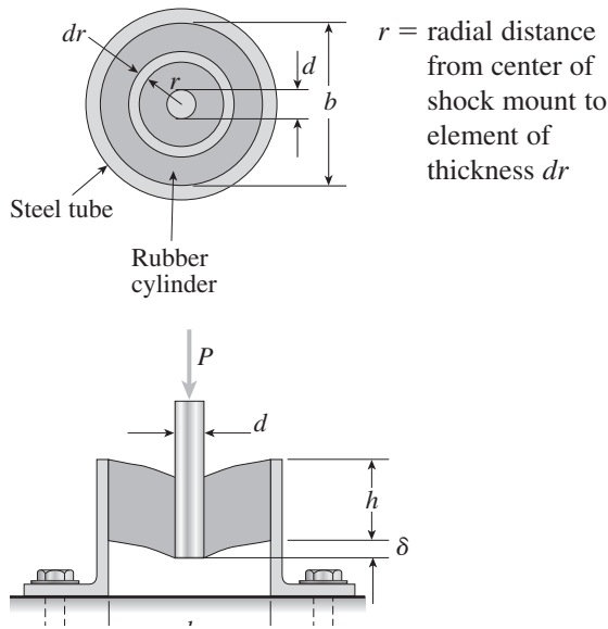
(a) SHEAR STRESS T AT RADIAL DISTANCE r
