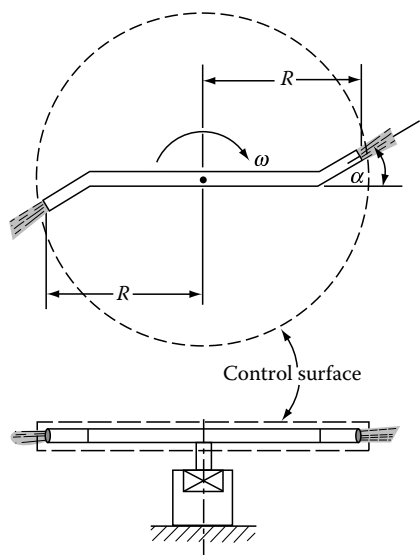
FIGURE 9.2 Lawn sprinkler of Example 9.1.
