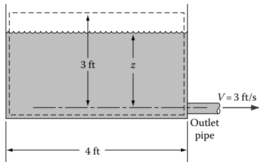
FIGURE 3.10 Circular tank of solvent being drained.
