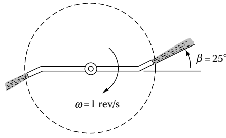
FIGURE 3.16 Plan view of a sprinkler head.
