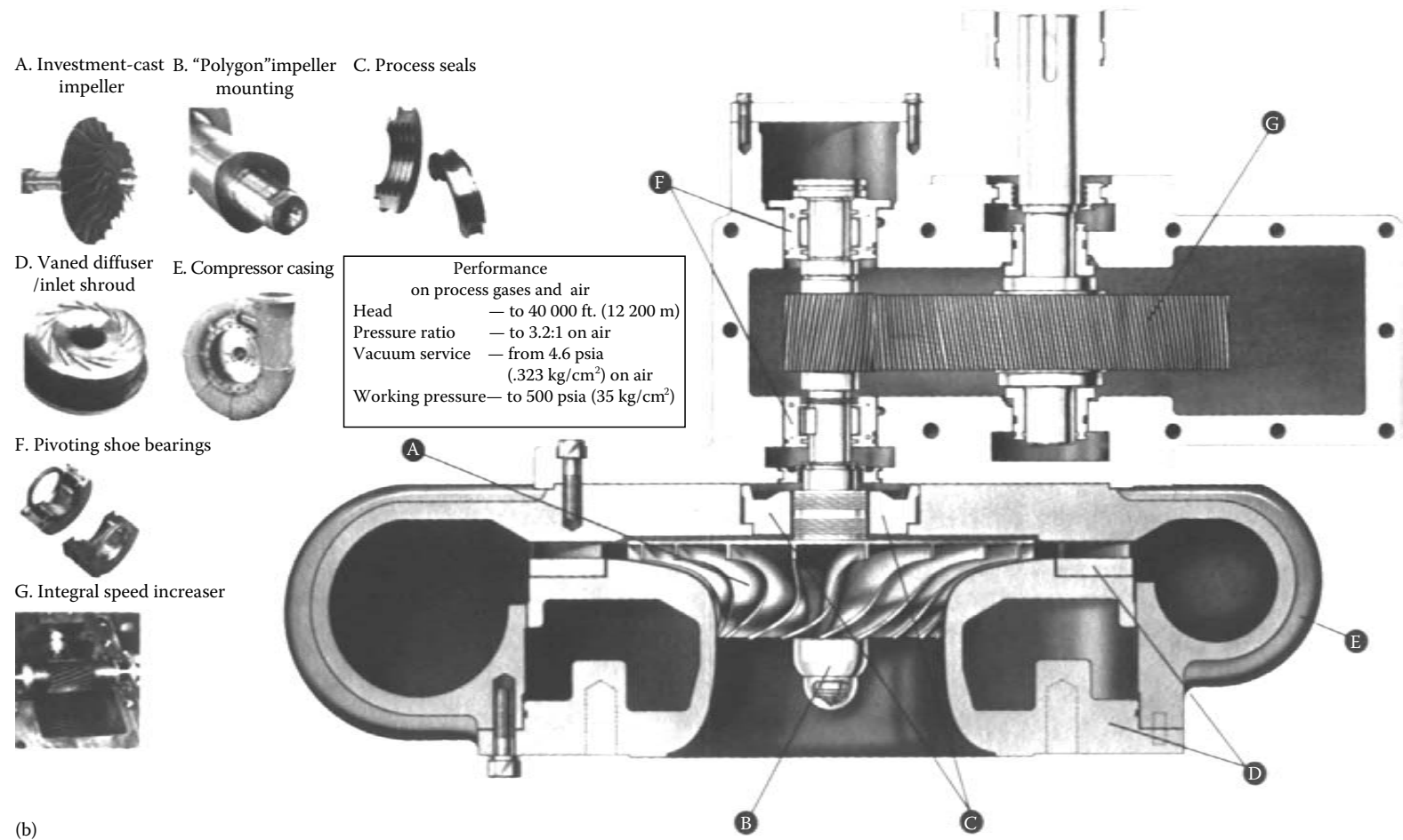
FIGURE 9.27 (continued) (b) A centrifugal compressor. (Courtesy of Atlas Copco Turbonetics Inc., Latham, NY.)
