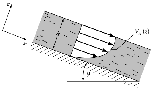
FIGURE 7.9 Laminar uniform open-channel flow.
