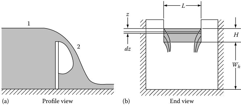
FIGURE 10.32 A contracted rectangular weir installed in a rectangular channel.
