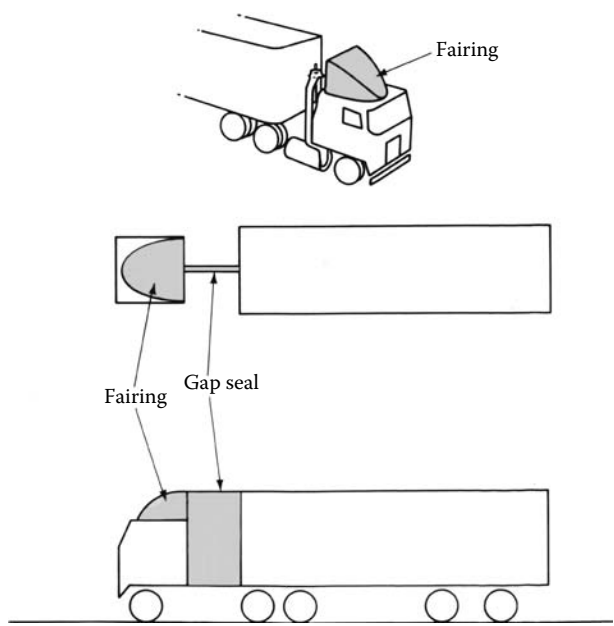
FIGURE 6.27 A fairing and gap seal attached to a tractor-trailer truck.
