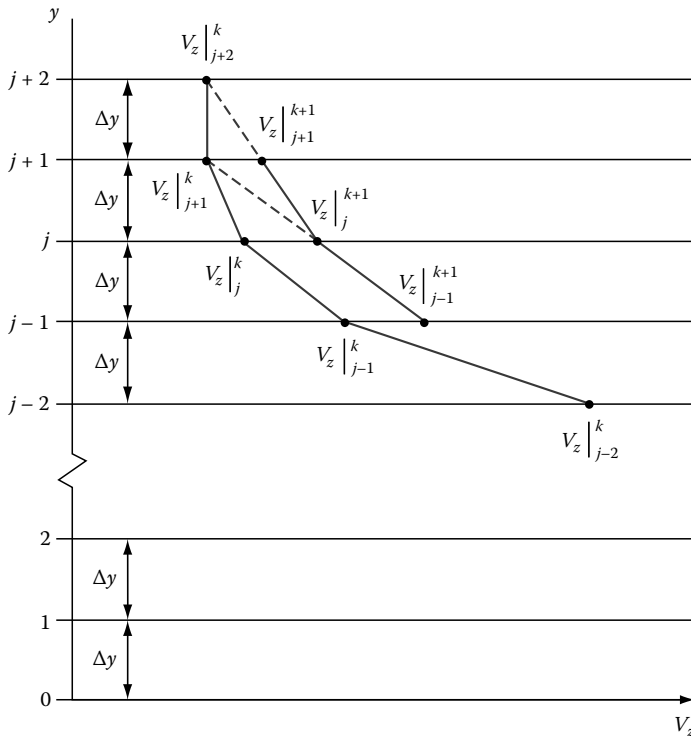
FIGURE 11.11 Graphical construction of Equation 11.33.
