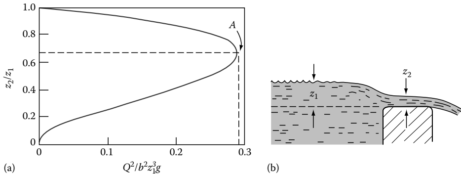
FIGURE 7.4 (a) A plot of the sluice gate equation for a rectangular channel and (b) flow over the crest of a dam.
