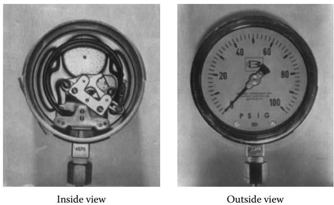
FIGURE 2.4 A bourdon-tube pressure gauge.
