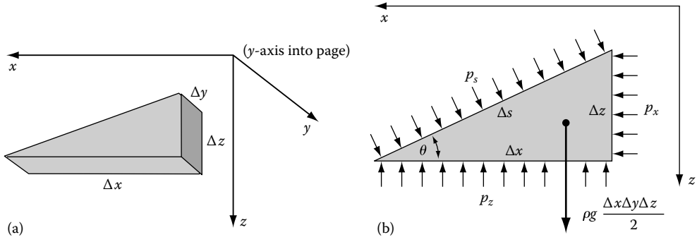
FIGURE 2.1 A wedge-shaped particle.
