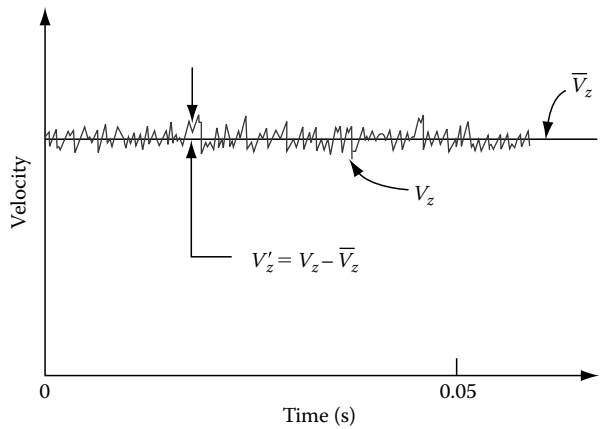
FIGURE 11.26 Velocity at a point in a turbulent flow.
