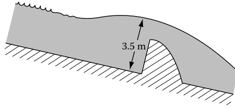
FIGURE 7.19 Backwater curve upstream of a dam.
