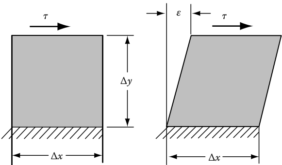
FIGURE 1.1 Deformation of a planar element.
