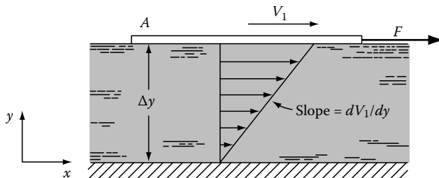
FIGURE 1.3 Shear stress applied to a fluid.
