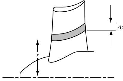
FIGURE 9.23 An incremental blade element.
