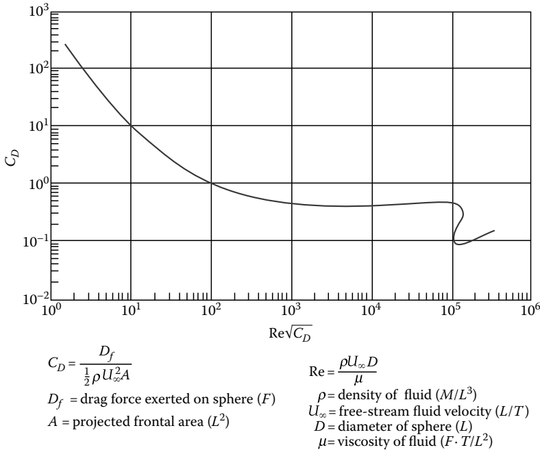
FIGURE 6.17 Drag coefficient as a function of \text{Re}\sqrt{C_D} for spheres. (Note on how this figure was developed: An enlarged copy of Figure 6.16 was scanned into a computer. The drawing was scaled and digitized to yield tabular data of C_D versus \text{Re} . The data were then manipulated appropriately to obtain \text{Re}\sqrt{C_D} , which was graphed versus C_D .)
