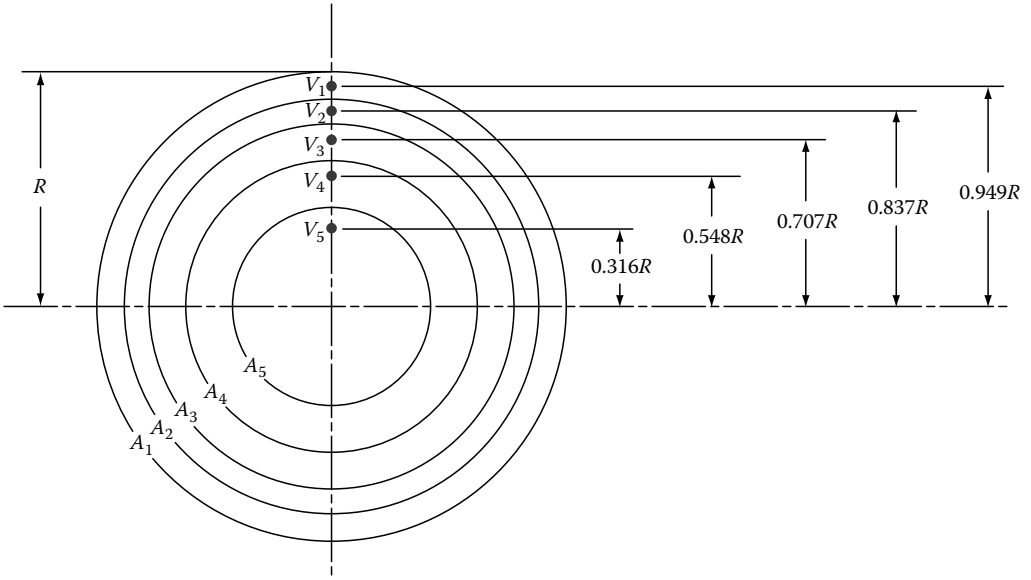
FIGURE 10.12 Circular cross section divided into five equal areas.
