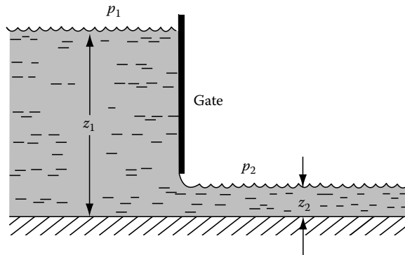
FIGURE 7.3 Flow under a sluice gate.
