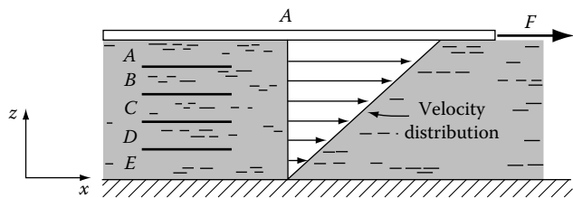
FIGURE 5.4 Layers of fluid flow between parallel plates.
