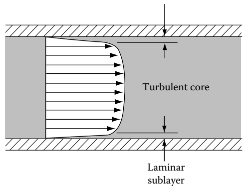
FIGURE 5.5 Laminar sublayer in turbulent pipe flow.
