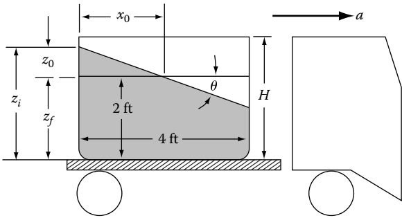
FIGURE 2.22 Accelerating truck with tank attached.
