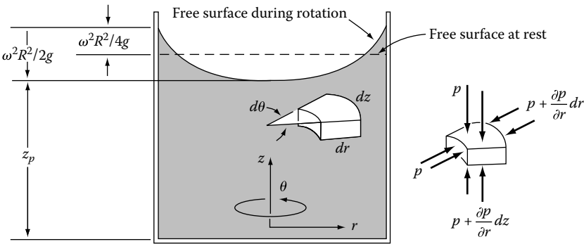
FIGURE 2.23 A rotating cylinder of radius R containing a liquid.
