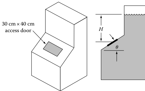
FIGURE 2.14 Ice container filled with liquid for Example 2.7.
