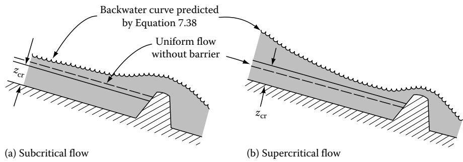
FIGURE 7.17 Flow upstream of a barrier.
