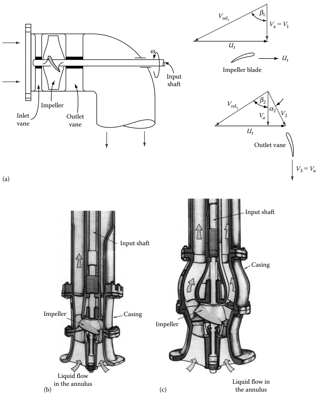
FIGURE 9.19 (a) Schematic of an axial-flow pump and the associated velocity diagram. (b) An axial-flow pump. (Courtesy of Fairbanks Morse Pump Division. With permission.) (c) A mixed-flow pump. (Courtesy of Fairbanks Morse Pump Division. With permission.)
