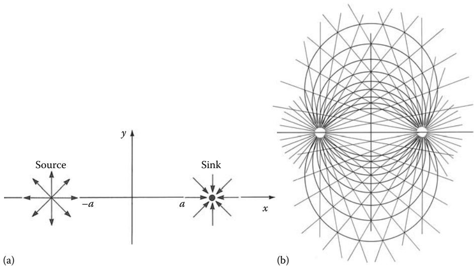
FIGURE 12.16 Streamlines of flow for a source and sink of equal strength. Centers of circles are located at the intersection of corresponding radial lines from source and sink. Each circle passes through both singularities.
