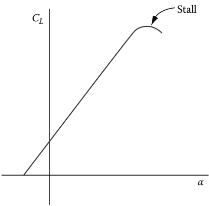
FIGURE 6.30 A typical plot of lift coefficient versus angle of attack for an airfoil.
