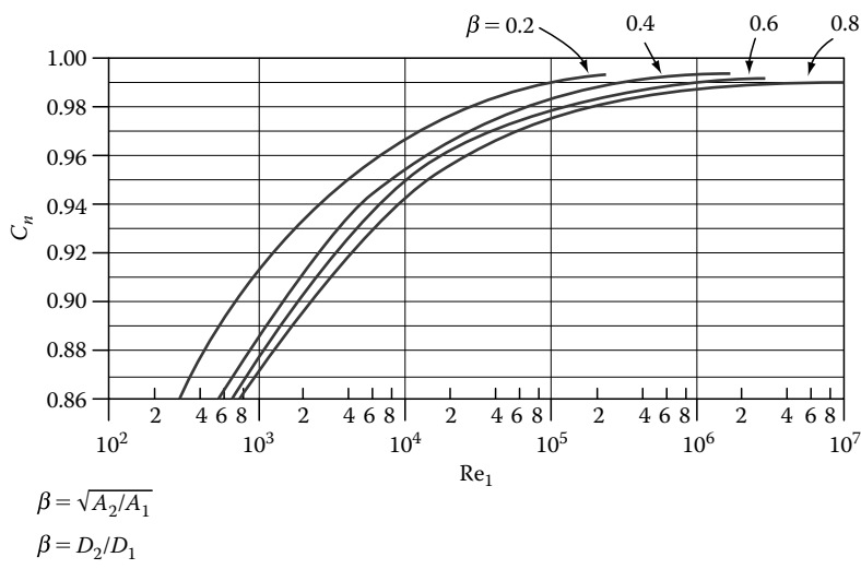
FIGURE 10.24 Discharge coefficient versus Reynolds number for flow nozzles. (Reprinted from Fluid Meters—Their Theory and Application , 5th edn., The American Society of Mechanical Engineers, New York, 1959. With permission.)
