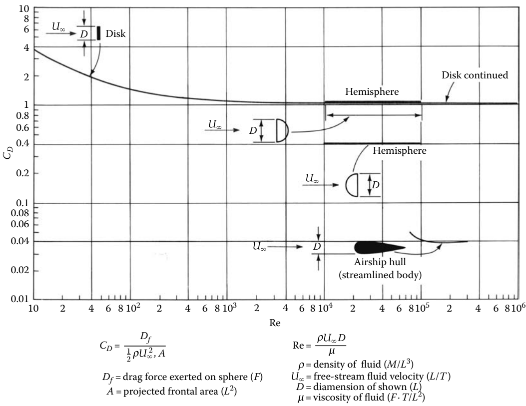
FIGURE 6.19 Drag coefficient versus Reynolds number for various three-dimensional bodies. (Data from various sources; see references at end of text.)
