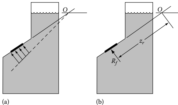
FIGURE 2.15 Profile views of container showing pressure prism, resultant force, and location.
