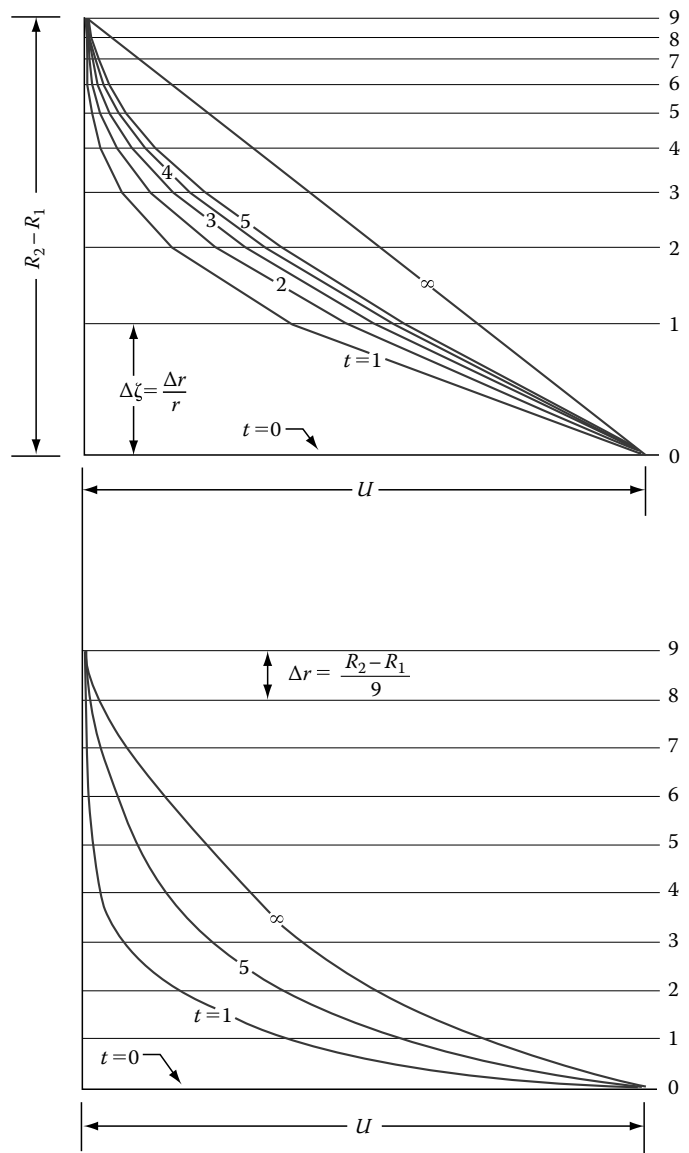
FIGURE 11.20 Solution to the problem of unsteady flow between two concentric cylinders.
