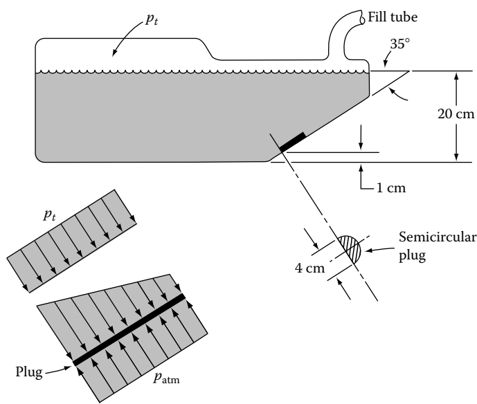
FIGURE 2.16 Sketch of a gas tank and plug for Example 2.8.
