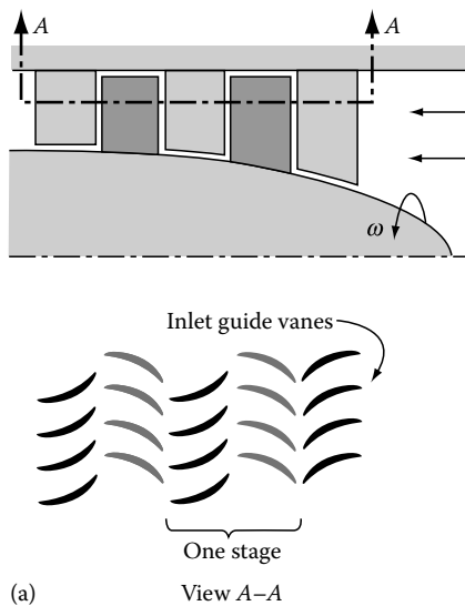
FIGURE 9.18 (a) An axial-flow compressor.
