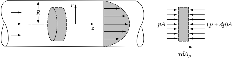
FIGURE 5.13 Laminar flow in a circular pipe.
