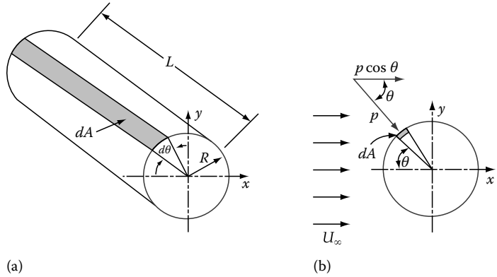
FIGURE 6.9 (a) Definition sketch of the area dA on a cylinder and (b) pressure p and its component, p \cos \theta , in the main flow direction.
