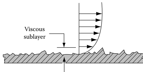
FIGURE 5.14 Turbulent flow in the vicinity of a wall.
