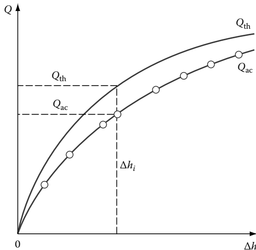
FIGURE 10.19 Flow rate versus pressure drop for a venturi meter.
