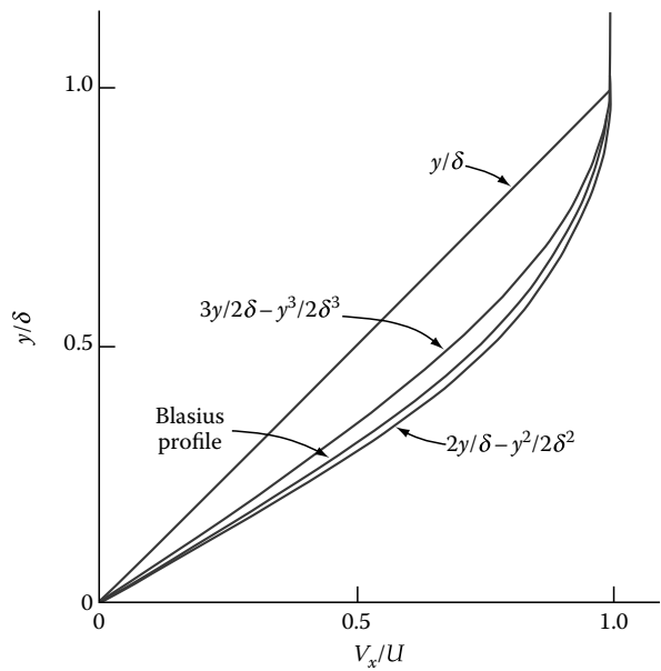
FIGURE 13.10 Blasius profile compared to the polynomial representations.
