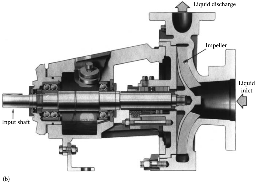
FIGURE 9.28 (continued) (b) Section view of a centrifugal pump and support housing (Courtesy of Allis-Chalmers Corp. With permission.)
