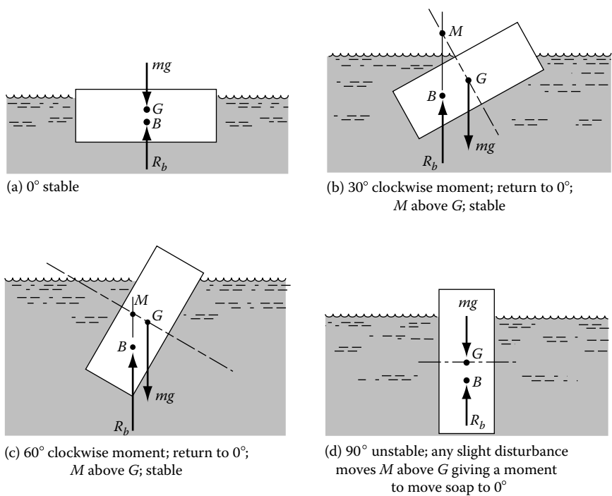
FIGURE 2.30 Solution to Example 2.15.
