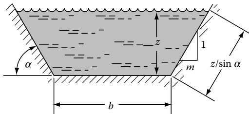
FIGURE 7.14 A trapezoidal cross section.
