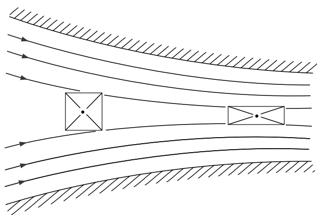
FIGURE 12.7 Irrotational flow through a converging duct.
