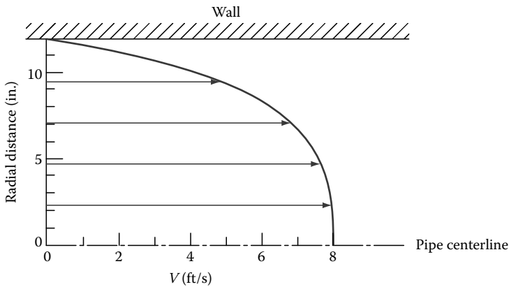
FIGURE 10.14 Velocity profile for ethyl alcohol in a pipe (Example 10.5).
