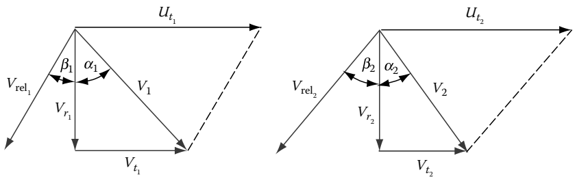
FIGURE 9.26 Velocity diagrams for a radial-flow turbine.
