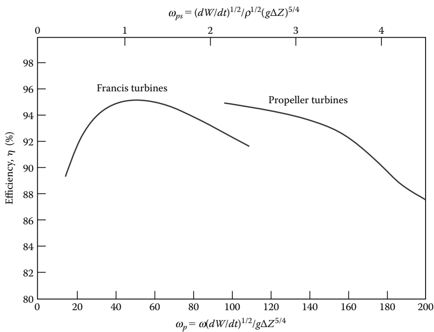
FIGURE 9.35 Hydraulic turbine efficiency ranges. (From Daugherty, R.L. and Franzini, J.B., Fluid Mechanics with Engineering Applications , 8th ed., McGraw-Hill Book Co., New York, 1977. With permission.)
