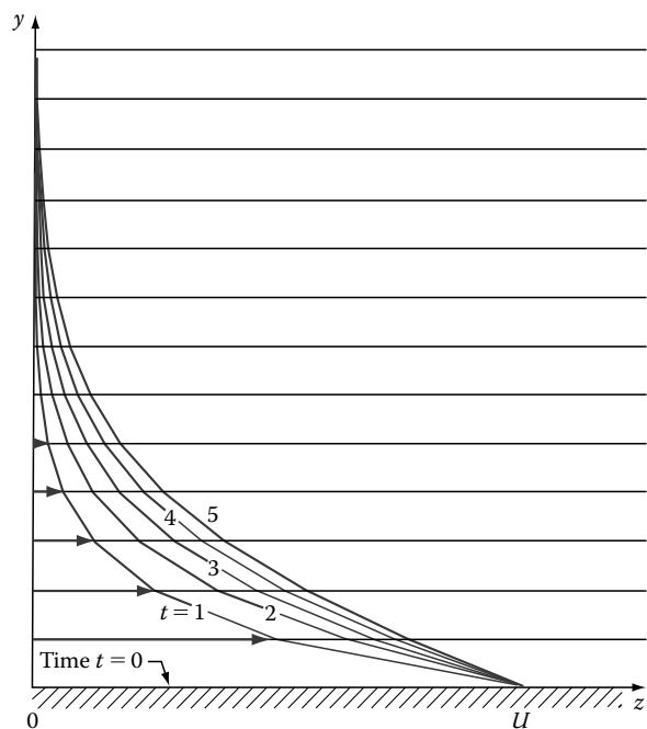
FIGURE 11.15 Solution for the velocity for the first five time intervals for the suddenly accelerated flat plate.
