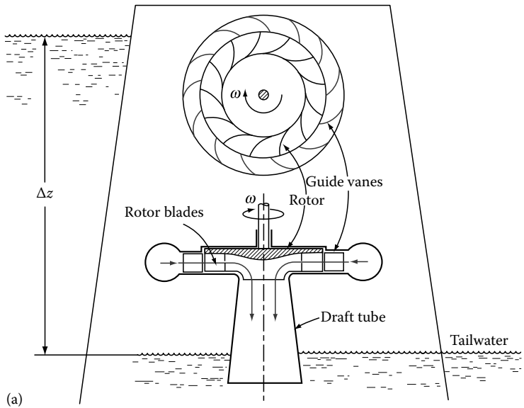
FIGURE 9.25 (a) A radial-flow turbine.
