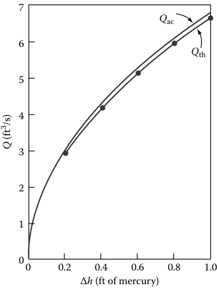
FIGURE 10.22 Calibration curve for the venturi meter of Example 10.6.
