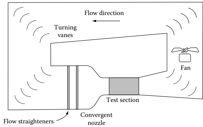
FIGURE 4.3 Schematic of a closed-loop wind tunnel.
