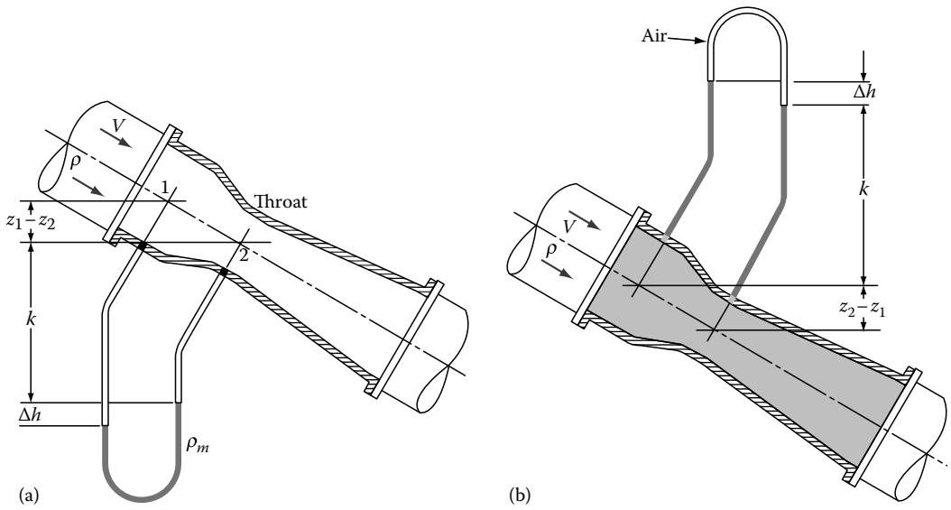
FIGURE 10.18 (a) A venturi meter with a two-liquid U-tube manometer. (b) A venturi meter with an inverted U-tube manometer.
