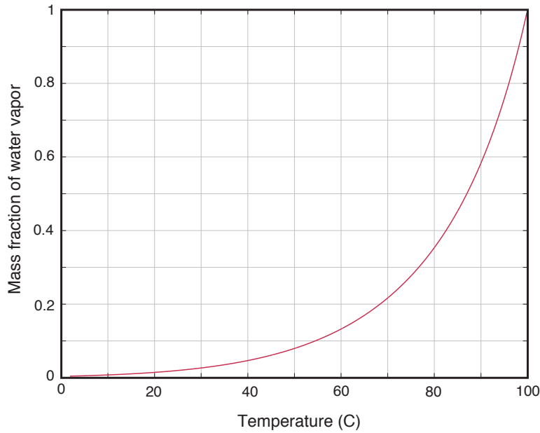
Figure 11.11 Mass fraction of water vapor in air adjacent to a liquid water (or tea) surface as a function of surface temperature (1 atm total pressure).
