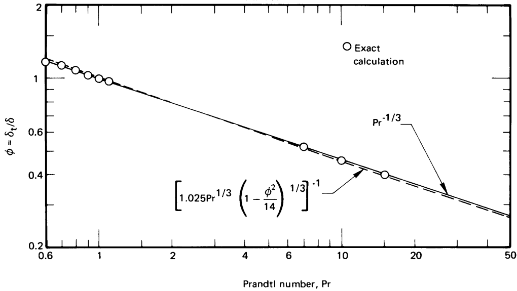
Figure 6.14 The exact and approximate Prandtl number influence on the ratio of b.l. thicknesses.
