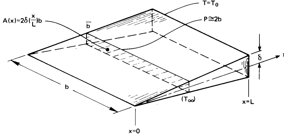
Figure 4.13 A two-dimensional wedge-shaped fin.
