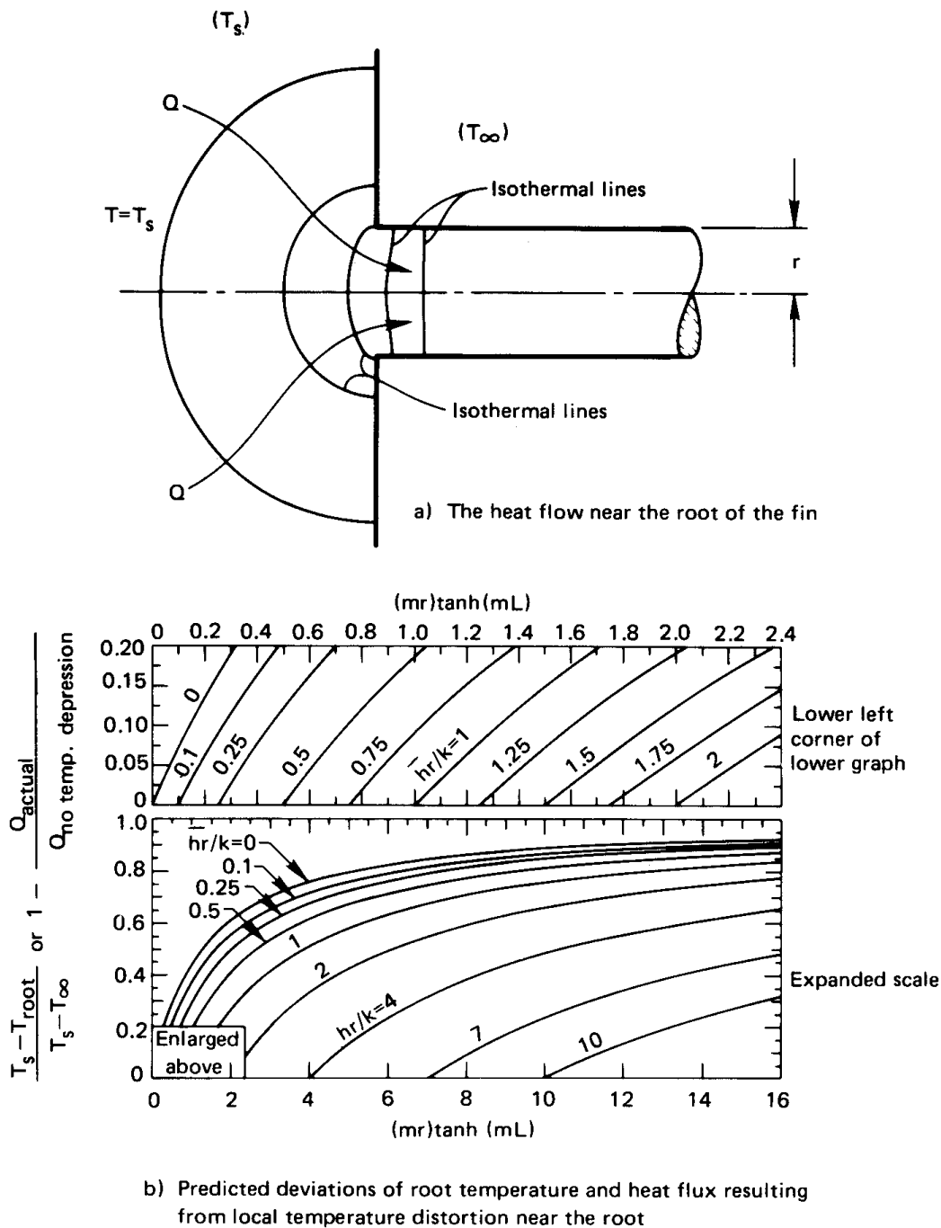
Figure 4.10 The influence of heat flow into the root of circular cylindrical fins [4.6]. This will be useful in fin design when \bar{h}r/k is less than about 1 (or \bar{h}A/kP is less than 1/2). The lines for larger values will not be needed for cooling fins.
