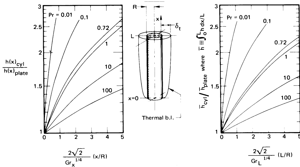
Figure 8.7 Corrections for h and \bar{h} on vertical isothermal plates to adapt them to vertical isothermal cylinders [8.11].
