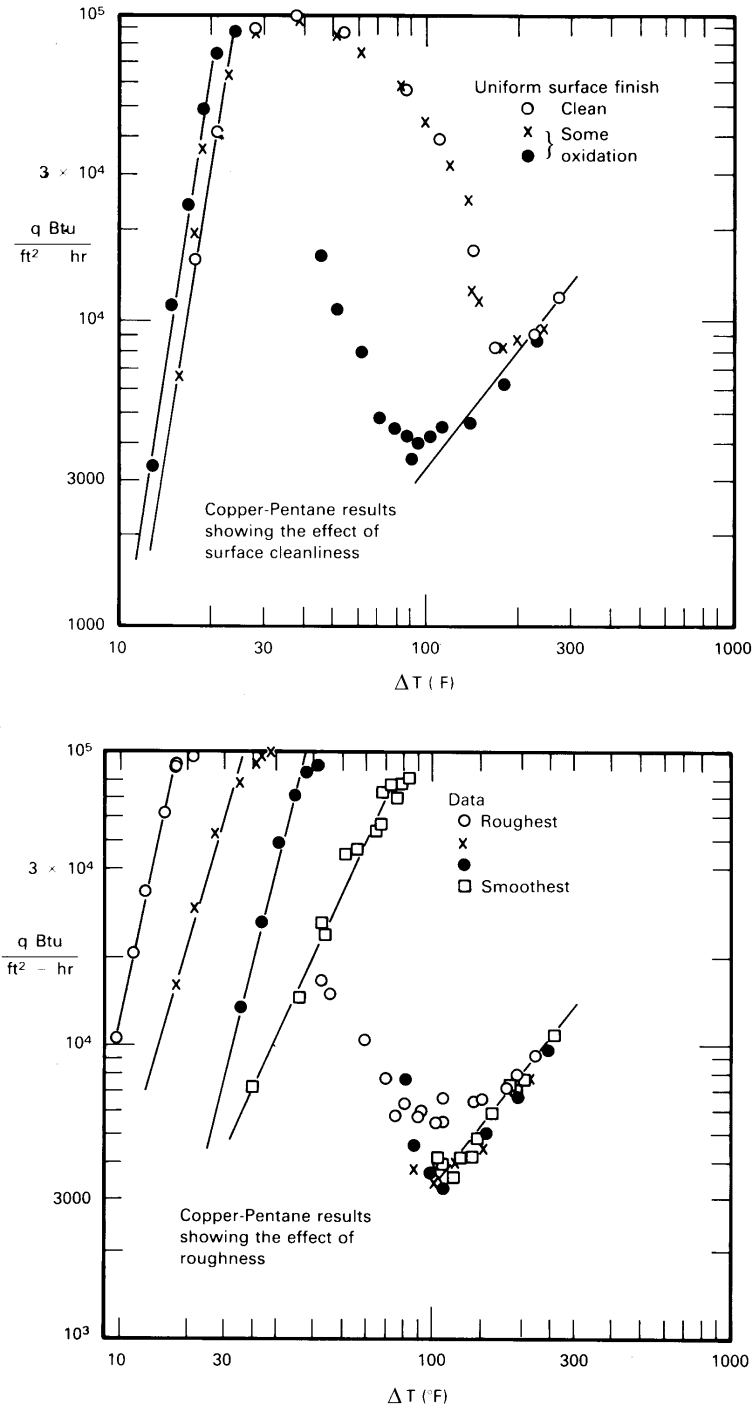
Figure 9.14 Typical data from Berenson's [9.30] study of the influence of surface condition on the boiling curve.
