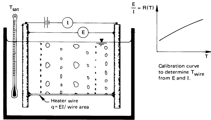
Nukiyama's experiment
