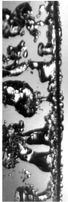
b. Two views of transitional boiling in acetone on a 0.32 cm diam. tube.
