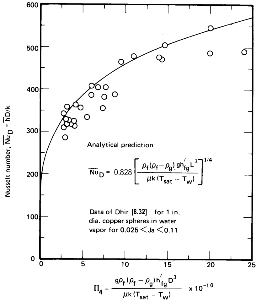
Figure 8.10 Correlation of the data of Dhira [8.32] for laminar film condensation on spheres at one value of Pr and for a range of \Pi_4 and Ja , with properties evaluated at (T_{\text{sat}} + T_w)/2 . Analytical prediction from [8.33].
