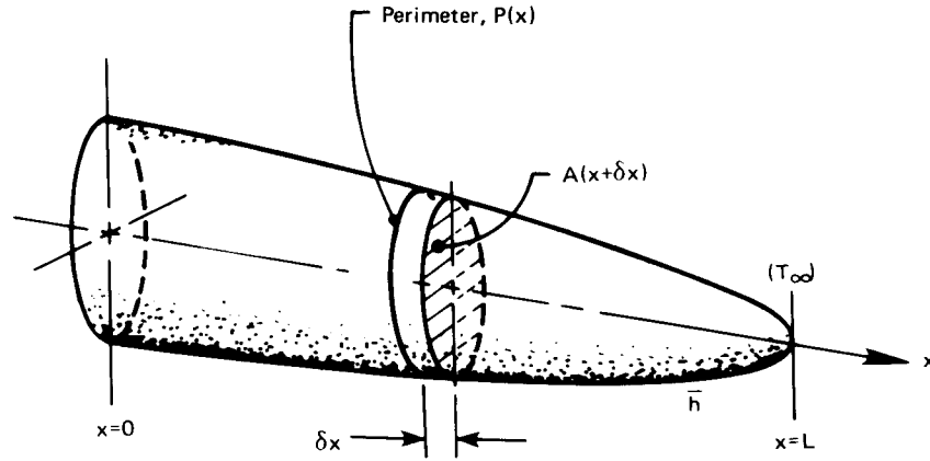
Figure 4.12 A general fin of variable cross section.
