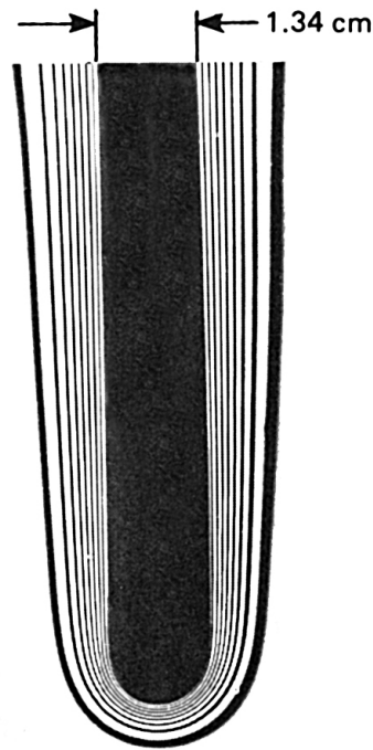
a. A 1.34 cm wide flat plate with a rounded leading edge in air. T_w = 46.5^\circ\text{C} , \Delta T = 17.0^\circ\text{C} , \text{Gr}_{\text{radius}} \approx 2250
