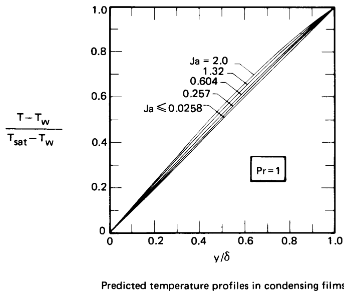
Figure 8.12 Results of the exact b.l. analysis of laminar film condensation on a vertical plate [8.36].
