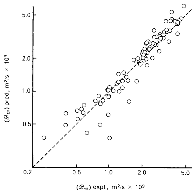
Figure 11.7 Comparison of liquid diffusion coefficients predicted by eqn. (11.50) with experimental values for assorted substances from [11.4].
